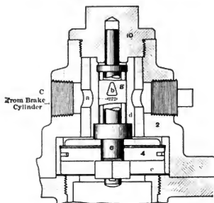
Fig. 2505. High-Speed Reducing Valve. Release Position.
